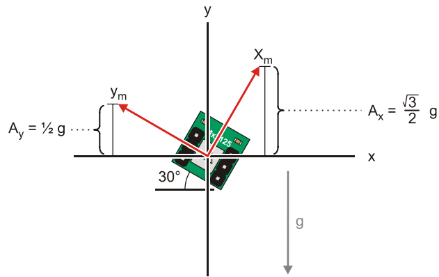
Figure 3-22: Accelerometer Rotated 30^\circ Clockwise
