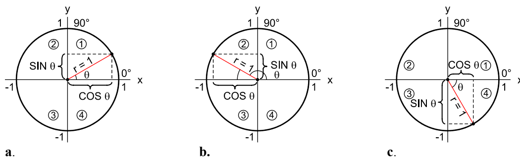
Figure 3-28: Unit Circle Sine and Cosine Examples
